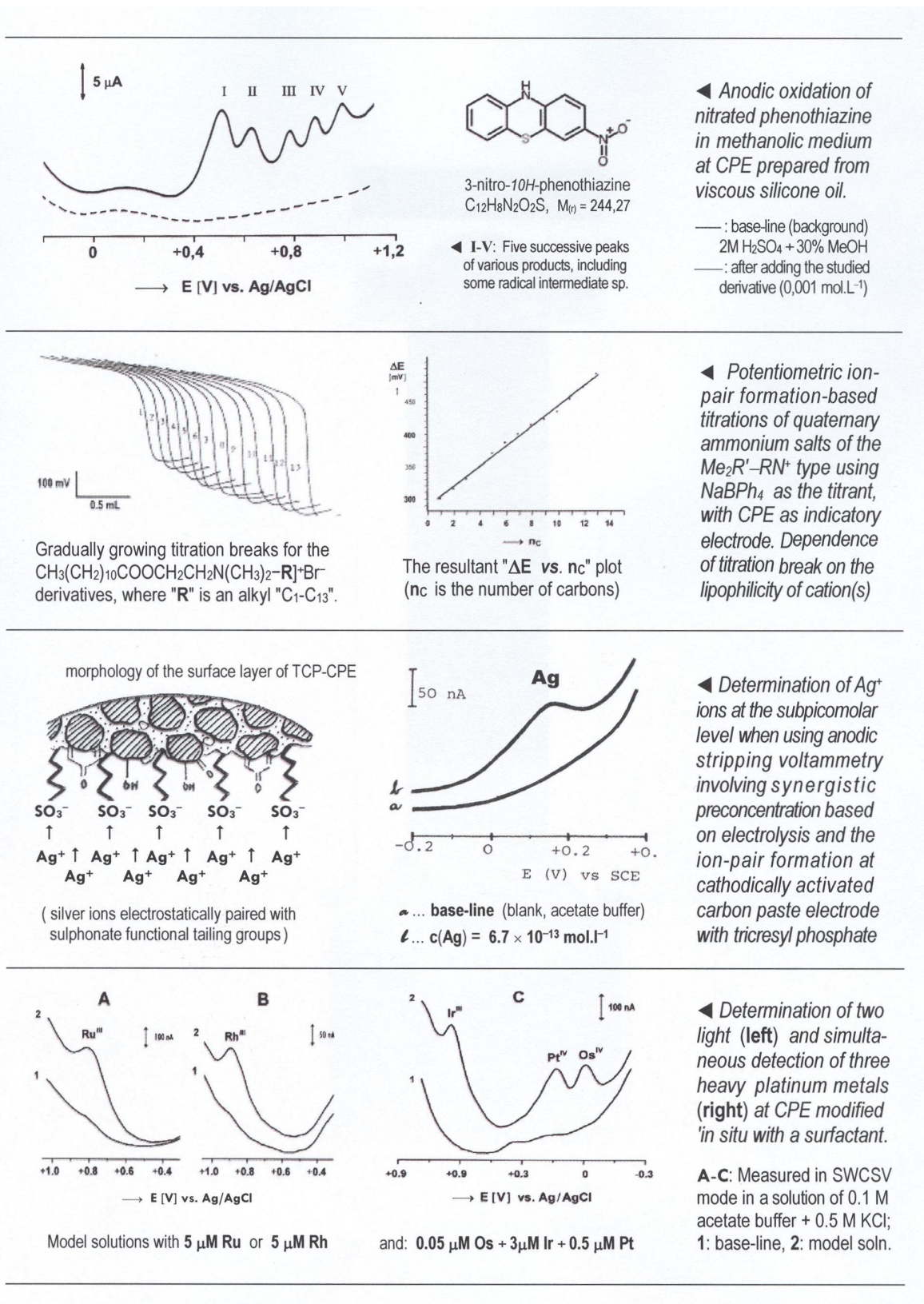
Fig. 5 Mosaic of some interesting measurements with carbon paste electrodes and related configurations (The individual images withdrawn from Refs [21,63,69,73,127,133,143] and eventually rearranged)
