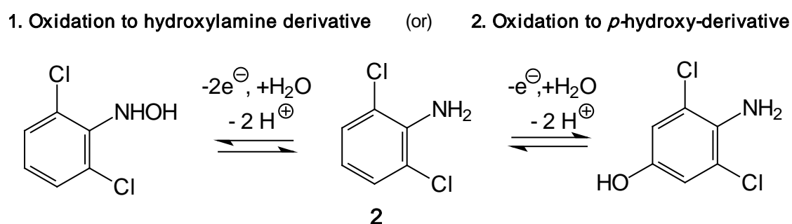
Fig. 5 Two possible pathways for the subsequent oxidation of 2
