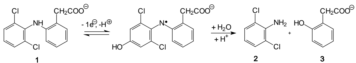
Fig. 3 Two-step mechanism of the electrode oxidation of Diclofenac (1) involving the formation of zwitterion and the subsequent hydrolysis to the final products 2,6-dichloroaniline (2) and salt of o -hydroxybenzeneacetic acid (3) (according to cit.[12])
