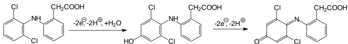
Fig. 2 Two-step mechanism of the electrode oxidation of Diclofenac involving the formation 5-OH derivative of Diclofenac and the subsequent quinone imine as the final product (according to cit.[11])
