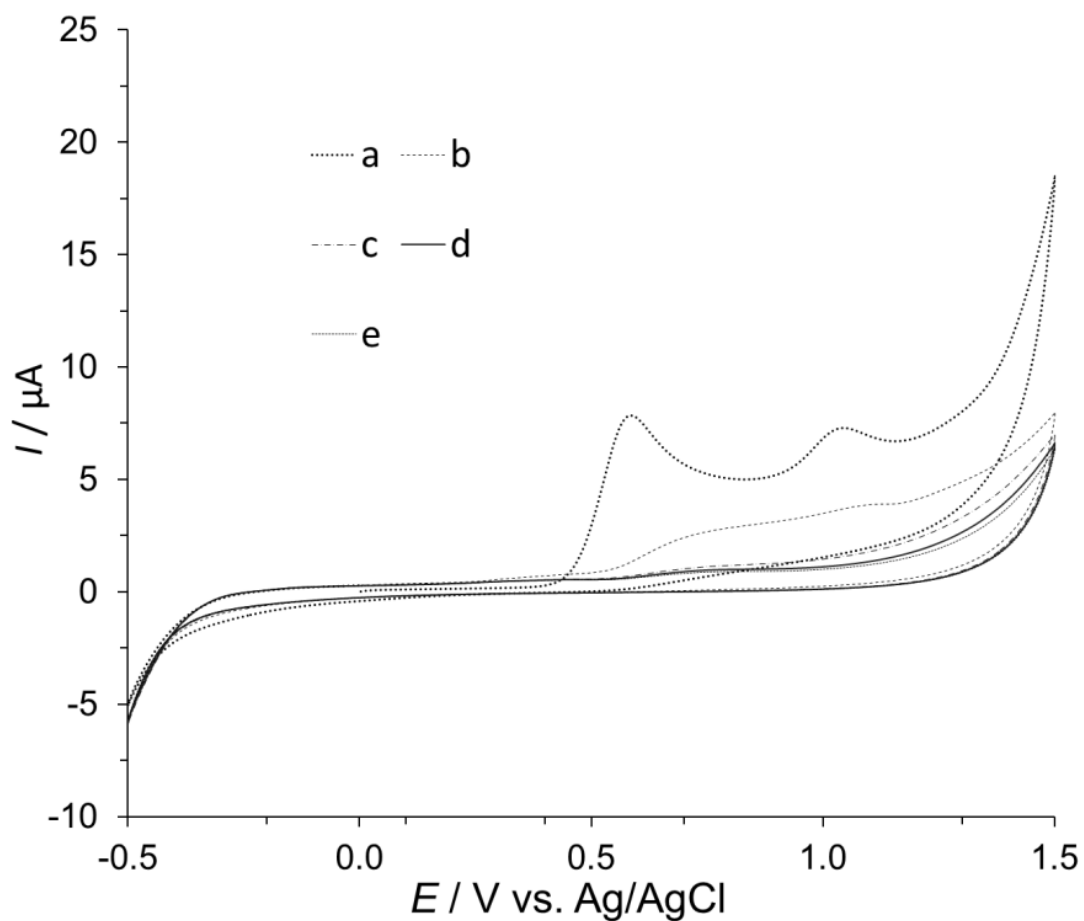
Fig. 4 Cyclic voltammetry of Diclofenac and two oxidation peaks within the potential range from -0.5 to 1.5 V vs. ref. Legend: a) 1 st anodic-cathodic cycle, b-e) other four cycles. Experimental conditions: CPE (unmodified), BRB (pH \sim 7 ), c = 5 \times 10^{-4} mol/dm 3 ; scan rate, 100 mV/s
