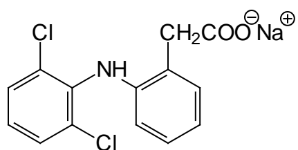
Fig. 1 Chemical structure of studied sodium salt of anti-inflammatory drug
