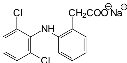
Fig. 1 Chemical structure of studied sodium salt of anti-inflammatory drug Diclofenac
