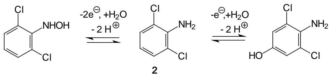
Fig. 5 Two possible pathways for the subsequent oxidation of 2
