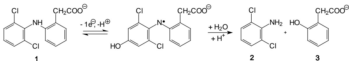
Fig. 3 Two-step mechanism of the electrode oxidation of Diclofenac ( 1 ) involving the formation of radical and the subsequent hydrolysis to the final
