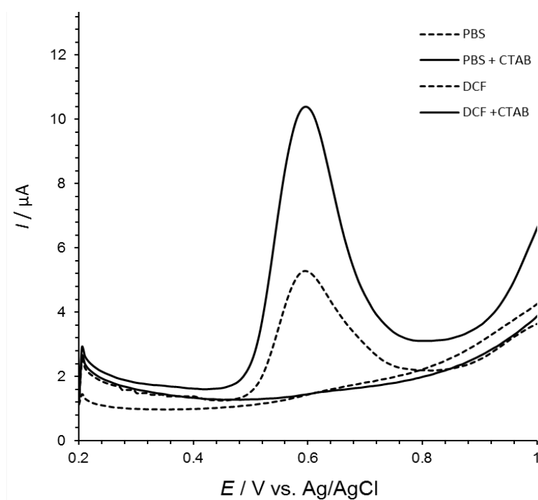
Fig. 6 The main oxidation peak of Diclofenac and the effect of the presence of CTAB surfactant in the (sample) solution. Legend: see both insets and quartet of steps of the experiment depicted. Experimental conditions: CPE; SWV; 0.1 M PBS + 100 \mu\text{M} CTAB; c(\text{Diclofenac}) = 5 \times 10^{-4} \text{ mol/dm}^3 ; potential scan: +0.2 \rightarrow 1.2 V vs. ref.; SW-ramp: frequency, f_{\text{sw}} = 60 \text{ Hz} , amplitude, E_{\text{sw}} = 40 \text{ mV} , potential step increment, p.i. = 5 mV
