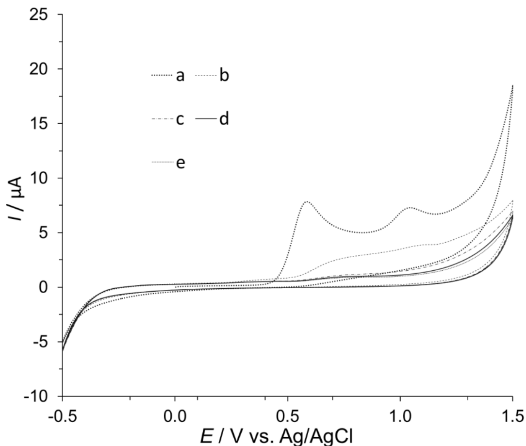
Fig. 4 Cyclic voltammetry of Diclofenac and two oxidation peaks within the potential range from -0.5 to 1.5 V vs. ref. Legend: a ) 1 st anodic-cathodic cycle, b-e ) other four cycles. Experimental conditions: CPE (unmodified), BRB (pH \sim 7 ), c (Diclofenac) = 5 \times 10^{-4} mol/dm 3 ; scan rate, 100 mV/s
