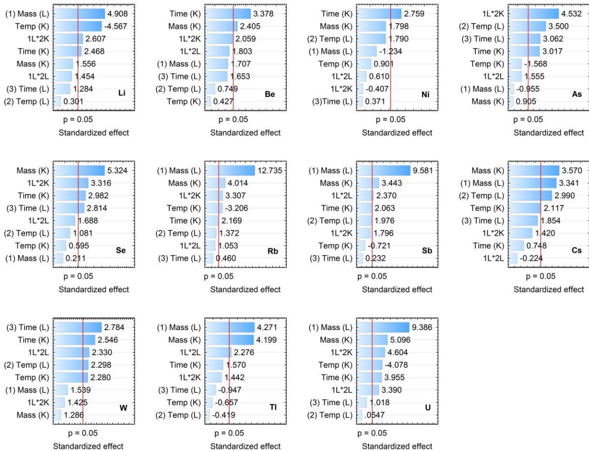
Fig. 1 Pareto charts of the standardized effects in the fractional factorial design 3^{3-1} for the study of variables (A) amount of \text{NH}_4\text{F} , (B) extraction temperature, (C) time and their interactions on extraction of selected elements. The L and Q letters indicate the linear and quadratic effect of the factor, respectively.
