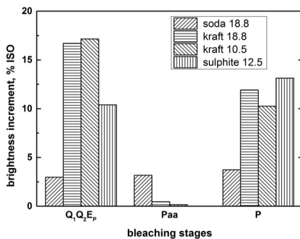
Fig. 2. Brightness increment in bleaching stages of Q 1 Q 2 E p PaaP sequence
