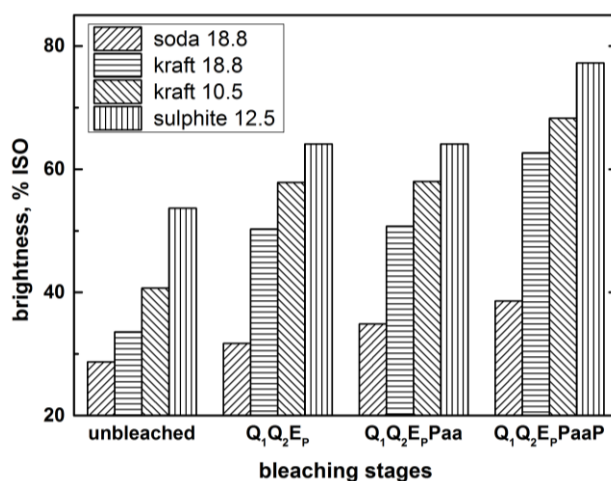
Fig. 1. Pulp brightness after bleaching stages
