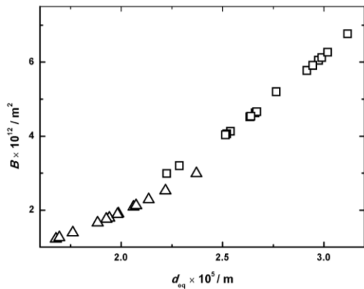
Fig. 1 Dependence of permeability on equivalent pore diameter for wash water at 25 °C. Pulp fibre bed: sulphite (□), kraft (△)
