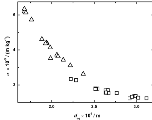
Fig. 2 Dependence of specific bed resistance on equivalent pore diameter for wash water (25 °C) flowing through sulphite (□) and kraft (△) pulp bed
