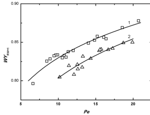
Fig. 4 Displacement wash yield as a function of the Péclet number for sulphite ( \square ) and kraft ( \triangle ) pulps. Eq. (7) (line 1), Eq. (8) (line 2)
