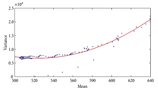
Figure 2. Mean–variance relationship
