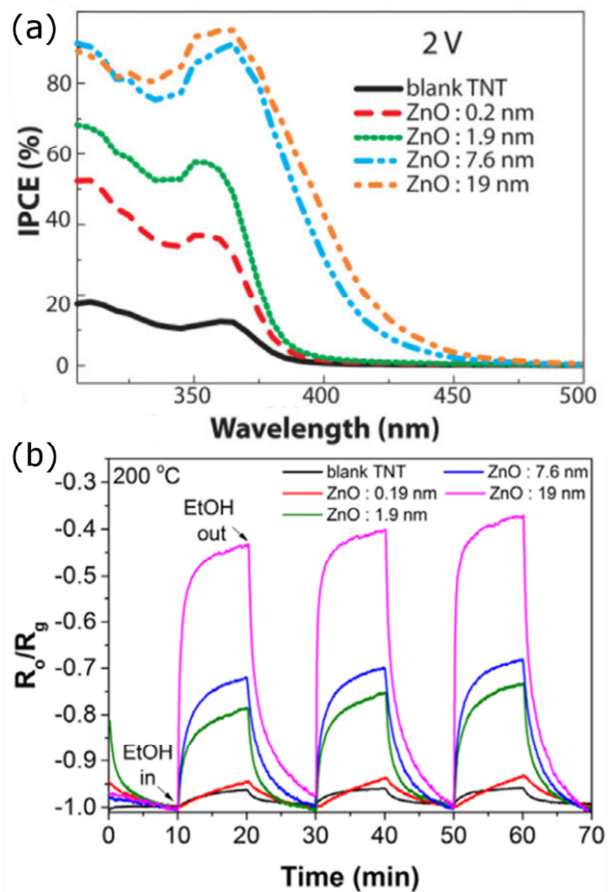
Figure 11: (a) Incident photon to electron conversion efficiency and (b) resistivity response upon exposure to ethanol of ALD ZnO coated TNT layers. Reproduced from [185].
