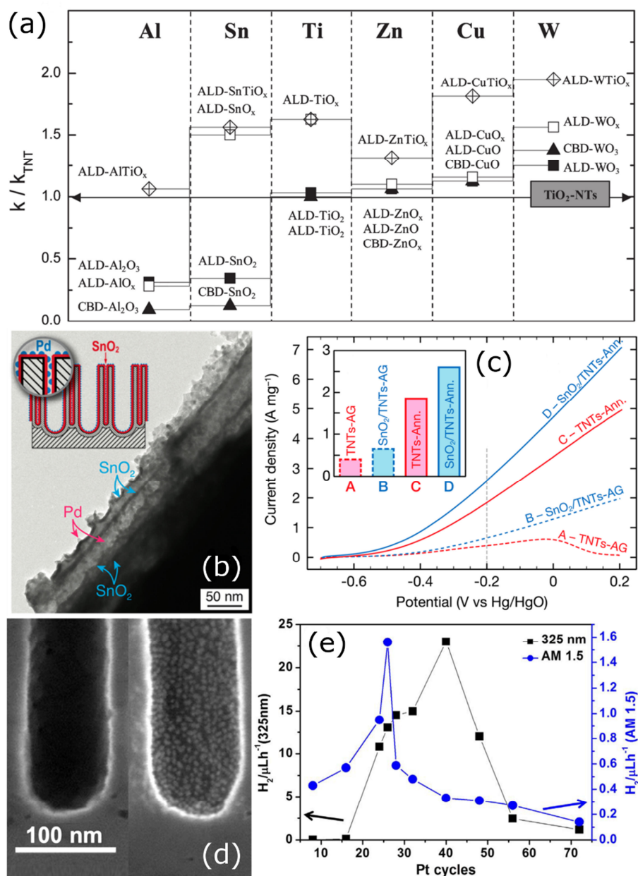
Figure 9: ALD functionalized TNT layers for photocatalytic and electrocatalytic applications. (a) Relative rate constants of methylene blue decomposition on TNT layers coated by various ALD and CBD deposited metal oxides/suboxides/mixed oxides, reproduced from [175]. (b) TEM image of ALD Pd nanoparticles on a ALD SnO 2 coated TNT layer for ethanol electrooxidation, composite nanostructure is illustrated schematically in the inset. (c) Linear sweep voltammetry and photocurrent density at -0.2 V (inset) for 500 cycles Pd on as-grown TNTs, annealed TNTs, as-grown SnO 2 /TNTs, and annealed SnO 2 /TNTs in 1 M KOH + 1 M C 2 H 5 OH, scan rate 25 mV/s. (b) and (c) were reproduced from [179]. (d) SEM picture of bare and 40 ALD cycles coated TNT and (e) corresponding dependence of photocatalytic H 2
