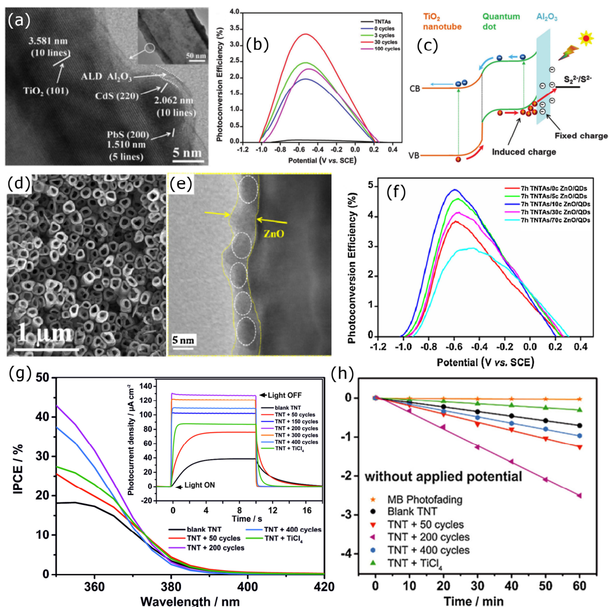
Figure 8: ALD deposited surface passivation layers for enhanced charge separation. (a) Representative TEM image, (b) observed PEC efficiency, and (c) model of interface band alignment of ALD \text{Al}_2\text{O}_3 passivated QD sensitized TNT layers, adopted from [141]. (d) SEM top view, (e) TEM side view, and (f) PEC efficiency of ALD ZnO coated QD sensitized TNT layers, reproduced from [146]. (g) IPCE and (h) rate of photocatalytic decomposition of model dye by ALD \text{TiO}_2 passivated TNT layers, reproduced from [149].
