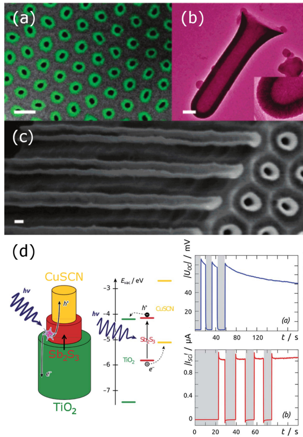
Figure 2: Illustration of functional nanostructures build on templates of porous alumina membranes utilizing ALD. (a)-(c) Micrographs (SEM and TEM) of ALD deposited iron oxide nanotubes for tunable magnetic properties, adopted from [69]. (d) ALD deposited TiO 2 (green) and Sb 2 S 3 (red) with (not ALD) CuSCN (yellow) in AAO for integration into photovoltaic device, reproduced from [81].
