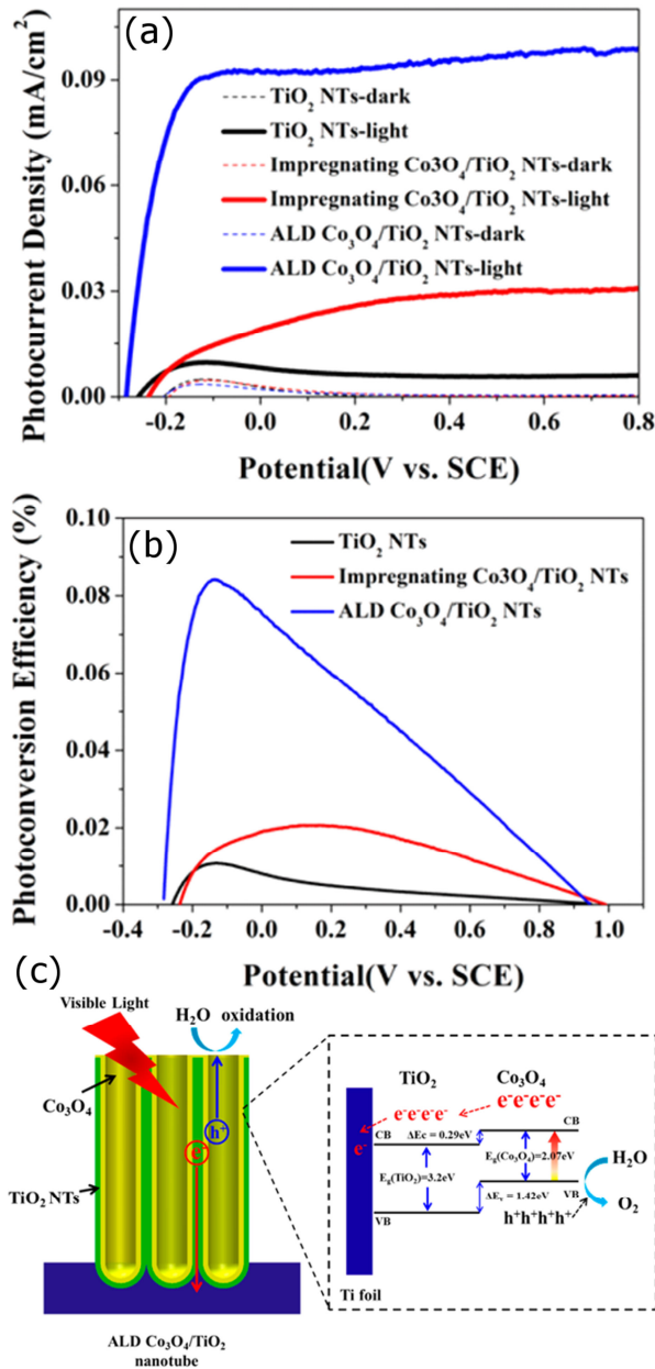
Figure 6: PEC performance of 4 nm thick Co 3 O 4 coating of TNT layers by ALD. (a) The photocurrent density and (b) photoconversion efficiency of Co 3 O 4 /TNT layer heterostructure upon visible-light illumination (> 420 nm, 100 mW/cm 2 ). (c) Illustration of band alignment within the heterostructure as determined by XPS. Reproduced from [128].
