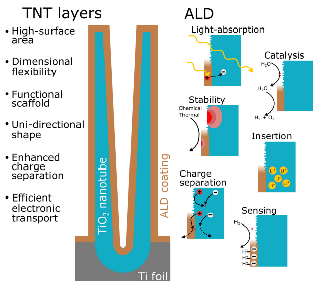
Figure 1: Illustration of utilization of ALD for advanced functionalization of TNT layers
