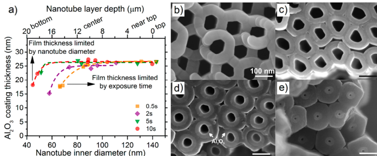
Figure 5: ALD Al 2 O 3 coating of TNT layers with aspect ratio of 180: (a) Influence of exposure time of TMA precursor during one ALD cycle on uniformity of thickness of Al 2 O 3 coating within TNT layer; (b-e) Illustration of uniform thickness of Al 2 O 3 coating for 5s TMA exposure time as revealed by SEM inspection through four different depth levels—top, near-top, middle, and bottom, respectively. Reproduced from [118].
