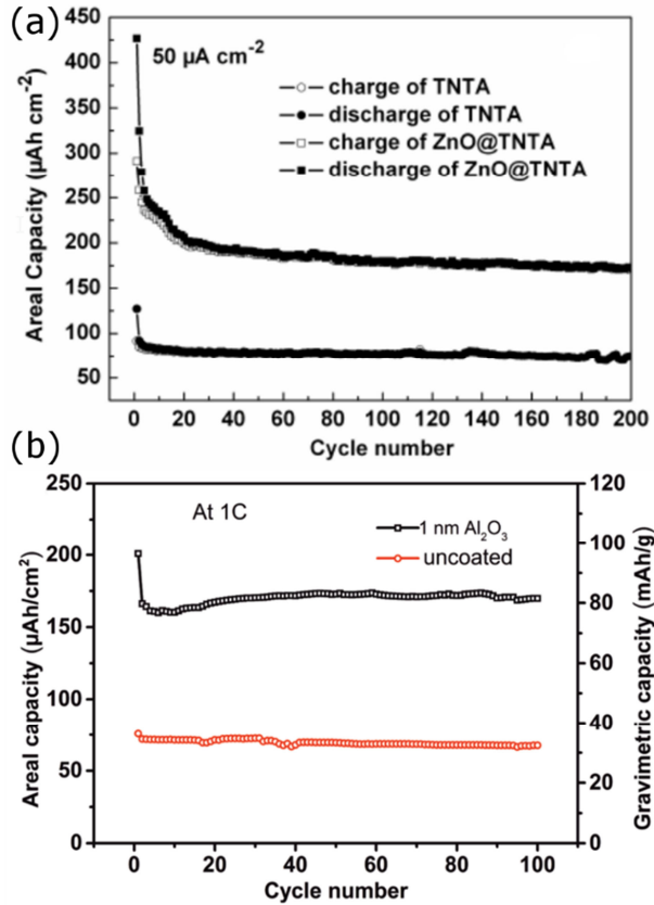
Figure 12: (a) Charge/discharge capacity of bare and ALD ZnO coated TNT layer as a function of charge/discharge cycles, reproduced from [200]. (b) Improved charge capacity of ALD \text{Al}_2\text{O}_3 coated TNT layer as compared with uncoated TNT layers throughout multiple charge/discharge cycles, reproduced from [201].
