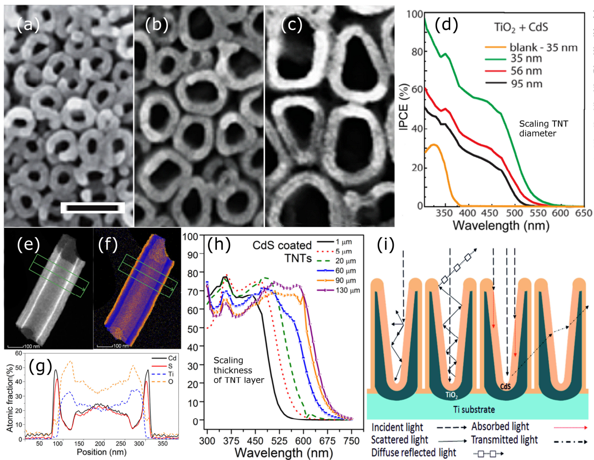
Figure 7: ALD coating of TNT layers by CdS light-absorber layer for improved visible-light photoresponse. (a-c) SEM images of 6 nm CdS coated TNT layers with average tube diameters 35 nm, 56 nm, and 95 nm, respectively, scale bar 100 nm. (d) IPCE of TNT layers with various nanotube diameter sensitized by 6 nm thick ALD CdS coating upon illumination with a monochromatized light source (e) High angle annular dark field (HAADF) STEM image and (f) STEM/EDX elemental map of fraction of nanotube coated by 10 nm thick CdS overlayer, the green arrows mark the corresponding elemental line profiles shown in (g). (h) IPCE of TNT layers with various thicknesses sensitized by 5 nm thick ALD CdS coating. (i) Illustration of multiple light scattering effects prolonging the optical path of light in TNT layer and facilitating efficient light harvesting. (a-d) Reproduced from [134] and (e-i) reproduced from [125].
