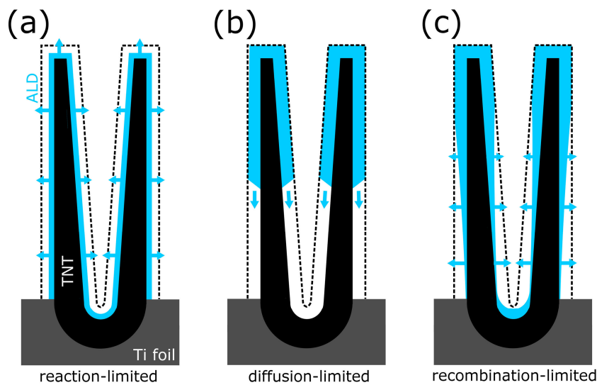
Figure 3: The illustration of evolution of step coverage profiles (light blue) of HAR nanostructure (black) by ALD under various process regimes. Light blue area and arrows indicate evolution of step coverage with increasing ALD exposure dose. Dashed black lines represent coverage profiles under saturated regime conditions (saturation exposure dose). (a) The reaction-limited, (b) the diffusion-limited, and (c) the recombination-limited regimes of ALD deposition.
