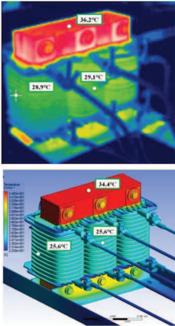
Fig. 14. Front view of temperature fields – steady state; air-flow 5 m s -1 . upper – thermovision screen lower – simulation
