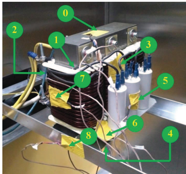
Fig. 13. Thermocouples positioning.
