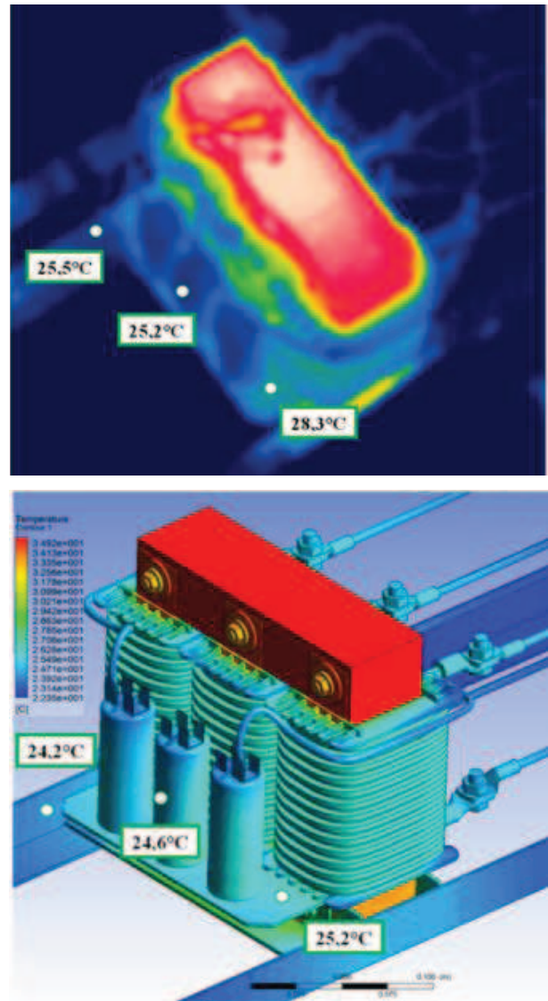
Fig. 15. Rear view of temperature fields – steady state; air-flow 5 m s -1 . upper – thermovision screen lower – simulation
