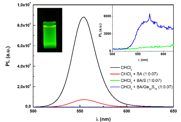
Fig. 5 PL spectra of \text{CdS}_{0.9}\text{Se}_{0.1} QDs in chloroform ( \text{CHCl}_3 ) with addition of various solutions. The left inset photo shows the \text{CdS}_{0.9}\text{Se}_{0.1} QDs - \text{CHCl}_3 solution under UV lamp light.
