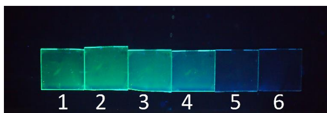
Fig. 11 The \text{CdS}_{0.9}\text{Se}_{0.1} QDs doped spin-coated \text{Ge}_{25}\text{S}_{75} thin films after 60 min UV exposure under UV lamp light. 1 – as-prepared thin film, 2 – annealed at 90 °C, 3 – annealed at 120 °C, 4 – annealed at 150 °C, 5 – annealed at 180 °C, 6 – annealed at 210 °C
