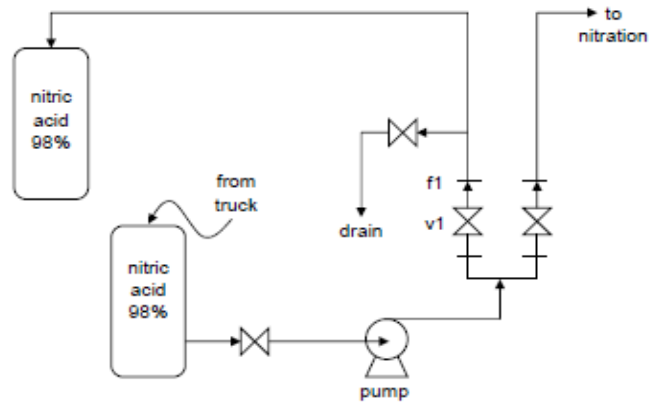
Figure 9. Nitric acid storage facility
