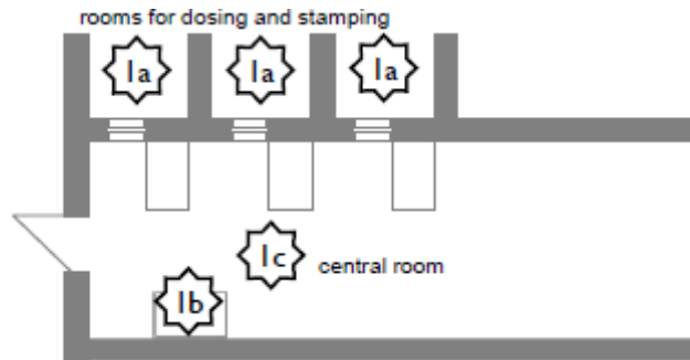
Figure 4. Hazards in the delay element production unit
