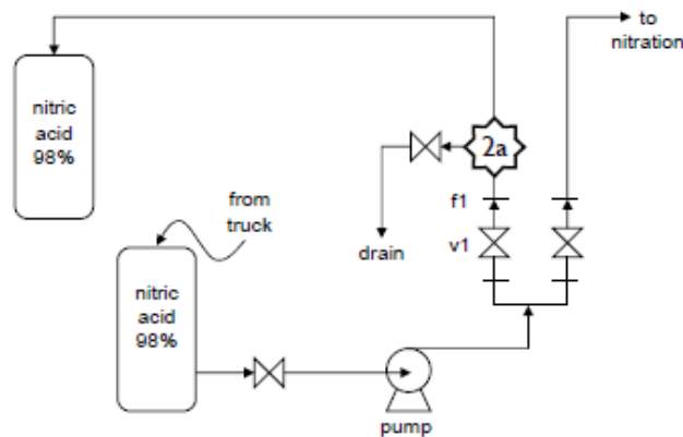
Figure 10. Selected hazard in nitric acid storage facility.
