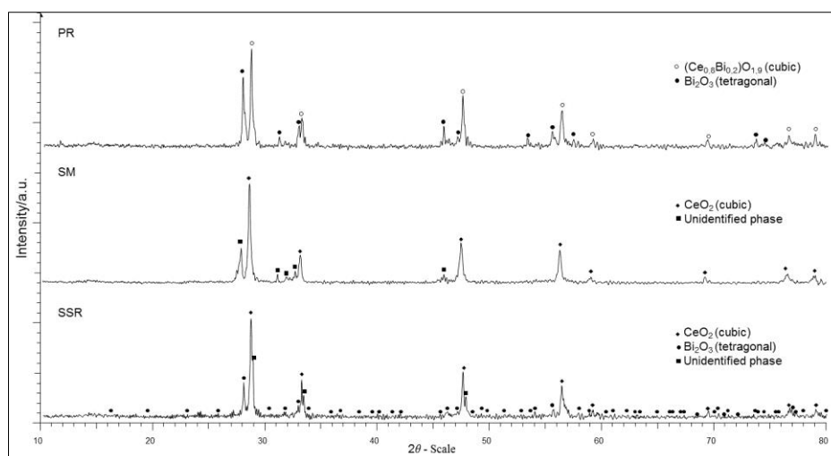
Fig. 1 Diffractograms of \text{Bi}_{1.5}\text{Zn}_{0.5}\text{Ce}_2\text{O}_7 pigments prepared by SSR, SM and PR ( 1000^\circ\text{C} )
