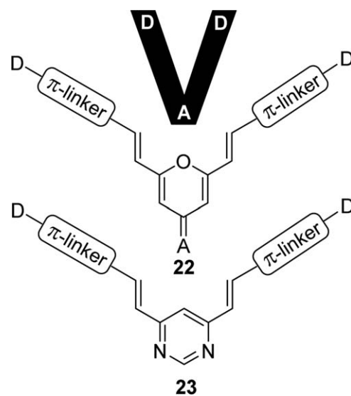
Fig. 10. Pyran- and diazine-derived V-shaped push-pull molecules.
