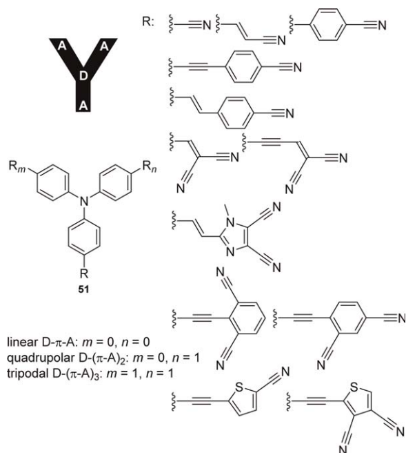
Fig. 18. TPA derivatives 51 with systematically altered peripheral (poly)cyano-substituted acceptor moieties.
